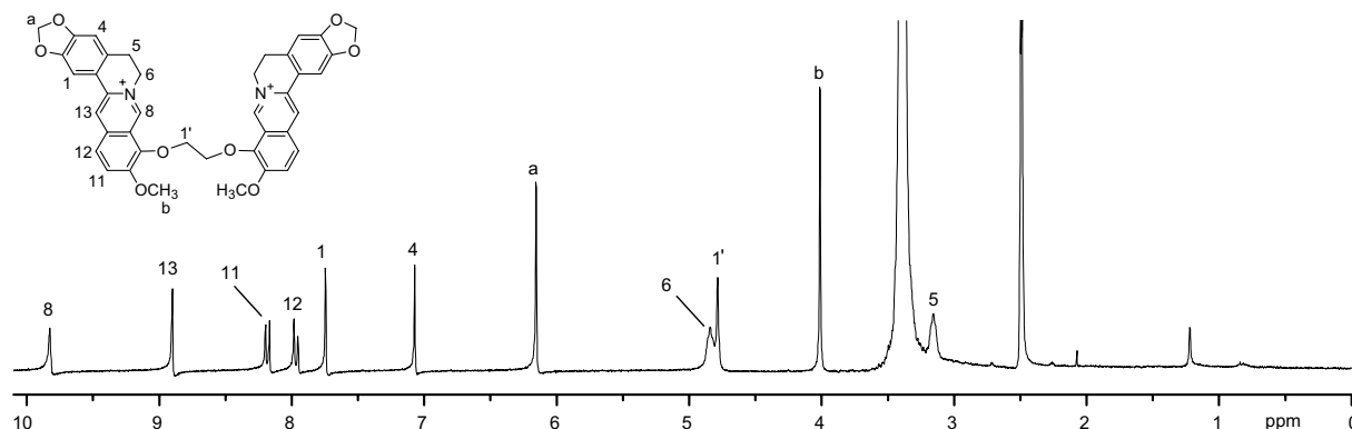
Figure 1. ^1H NMR (300 MHz) spectrum of 3a in DMSO-d_6 .
