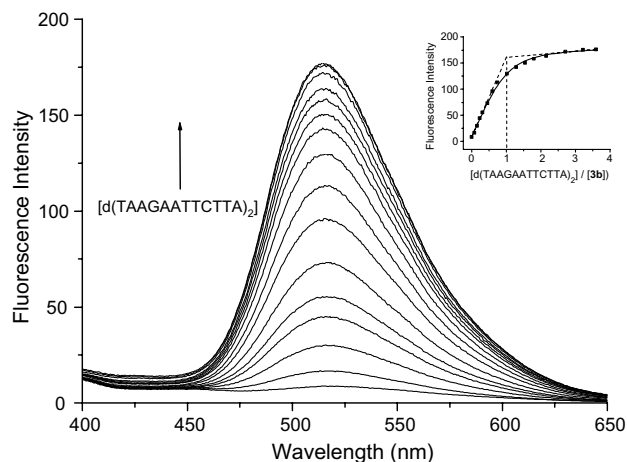
Figure 2. Fluorescence spectra of 3b ( 2.47 \times 10^{-6} M) with d(TAAGAATTCTTA)_2 of increasing concentrations ( 0–8.89 \times 10^{-6} M) in 50 mM Tris-HCl (pH 6.35) at room temperature, ex 355 nm. The inset indicates the relationship between the fluorescence intensities (at em 516.7 nm) and the molar ratio of d(TAAGAATTCTTA)_2 to 3b .
